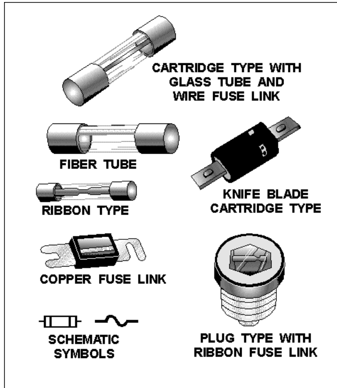
Figure 2-1.—Typical fuses and schematic symbols.
